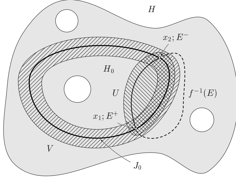
Figure 3: Arcs and loops in H
