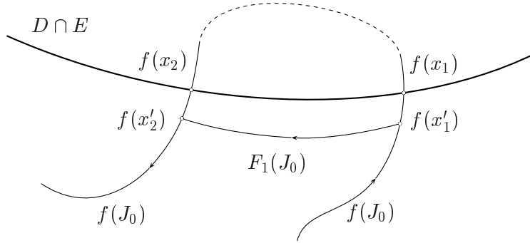
Figure 4: A modification of f
